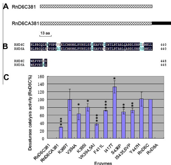
Fig. 1. Schematic structural diagrams and desaturation activities of the mutated proteins relative to RnD6C activity. (A) Schematic structural diagrams of RnD6C381 and RnD6CA381. Regions in originate from RnD6C, and regions in black are substituted from the corresponding region of RnD8A. (B) Schematic structural diagrams of RnD6C C-terminal mutation sites. (C) Desaturation activities of the mutated proteins relative to RnD6C activity. Conversion rates of mutated proteins in yeast were analyzed for the fatty acid LA following a 72 h induction. For comparison, the mean conversion rate of RnD6C was defined as 100%. Values are the mean of three independent assays \pm SD. t -test: * P < 0.05, ** P < 0.01, *** P < 0.0005.
